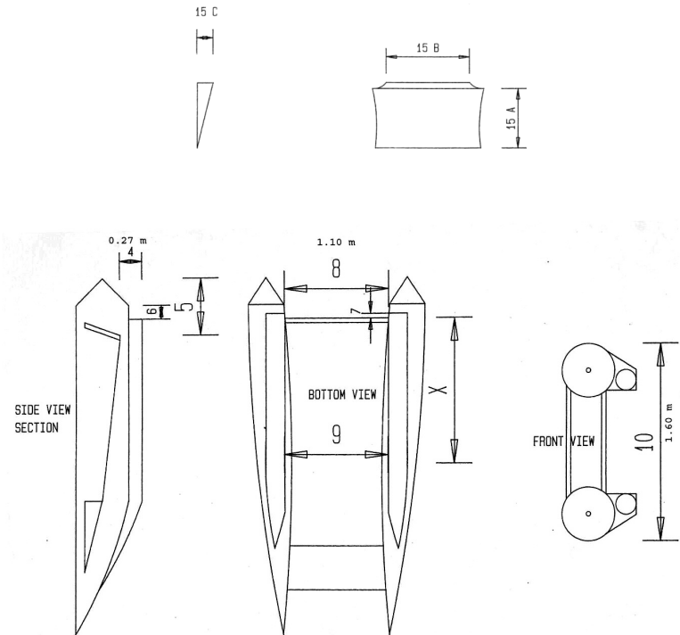
HULL DIAGRAM B:
