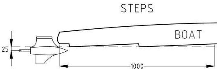
HYDROPLANE PROPELLER SHAFT HEIGHT MEASUREMENTS
